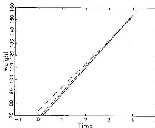
Fig. 3. Typical growth curve for data taken from ref. 18. Lines shown are for rat No. 8. (—) Submodel; (---) individual estimate; (- - -) EB estimate.
