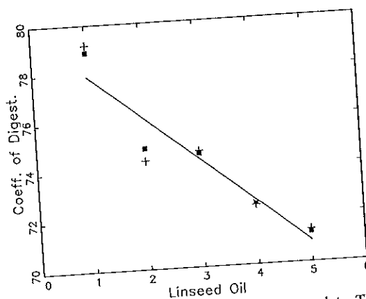
Fig. 2. Estimates of the cell means for the steer data. The line represents the submodel \hat{\theta} = 79.66 - 1.76X . The crosses are the cell means, and the squares are the EB estimates.
