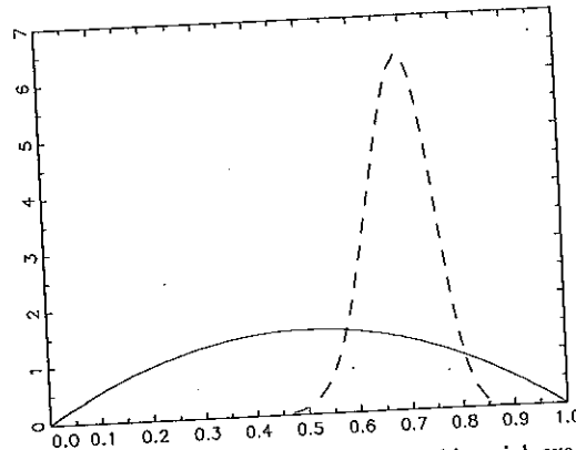
Fig. 1. Bayes prior and posterior for binomial example of Section 4.1. The solid line is \pi(p) and the dashed line is \pi(p|y) .
