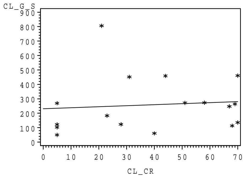
Figure 7.1: Plot of gemfibrozil vs creatinine clearance at single dose, and estimated regression line ( \hat{y} = 231.31 + 0.71x )
