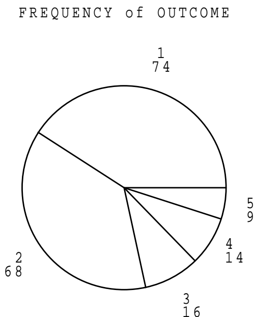
Figure 1.3: Pie Chart of frequency of each outcome in antibiotic study
