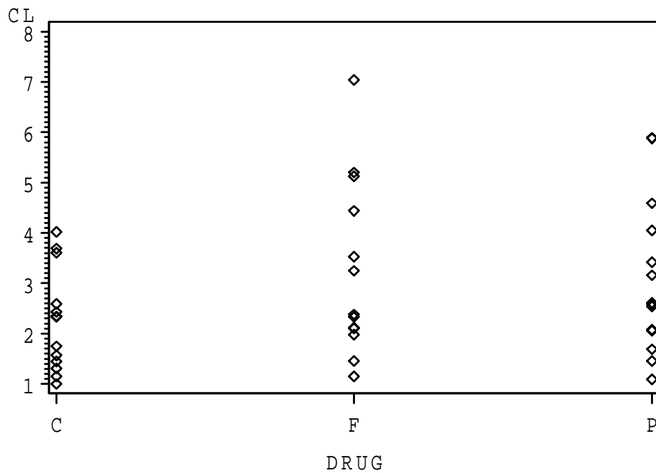
Figure 1.6: Plot of theophylline clearance vs interacting drug
