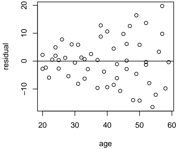
Residual Plot
