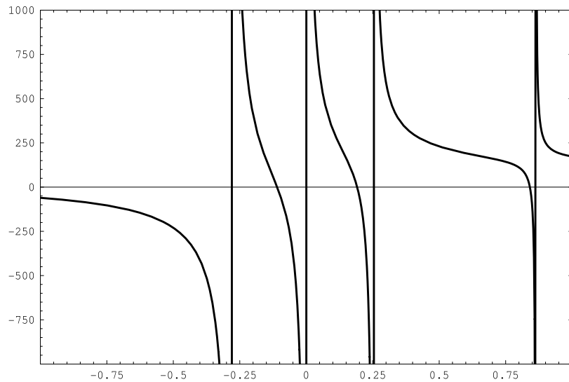
Fig. 1. For \mathbf{n} = \{10, 7, 5, 2, 1\} , a graph of the left side of (13) as a function of r_j , with j = 2 .
